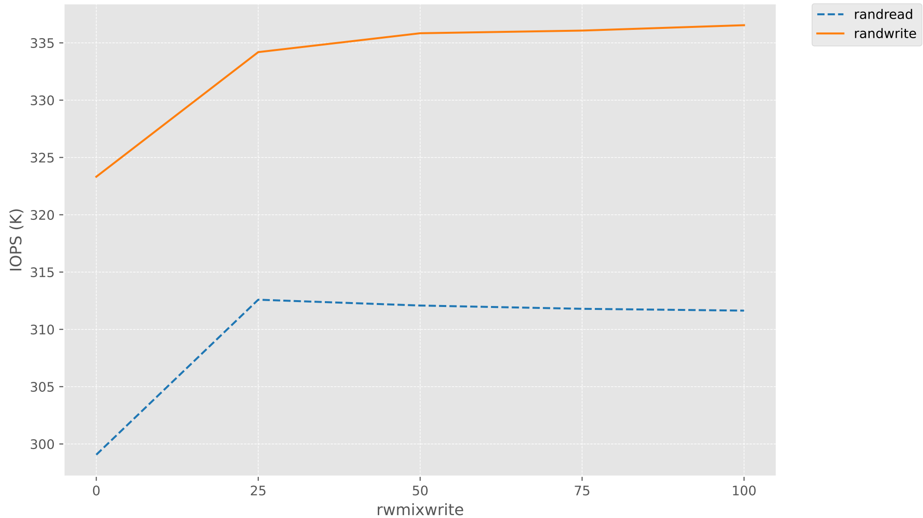
IOPS vs rwmixwrite
